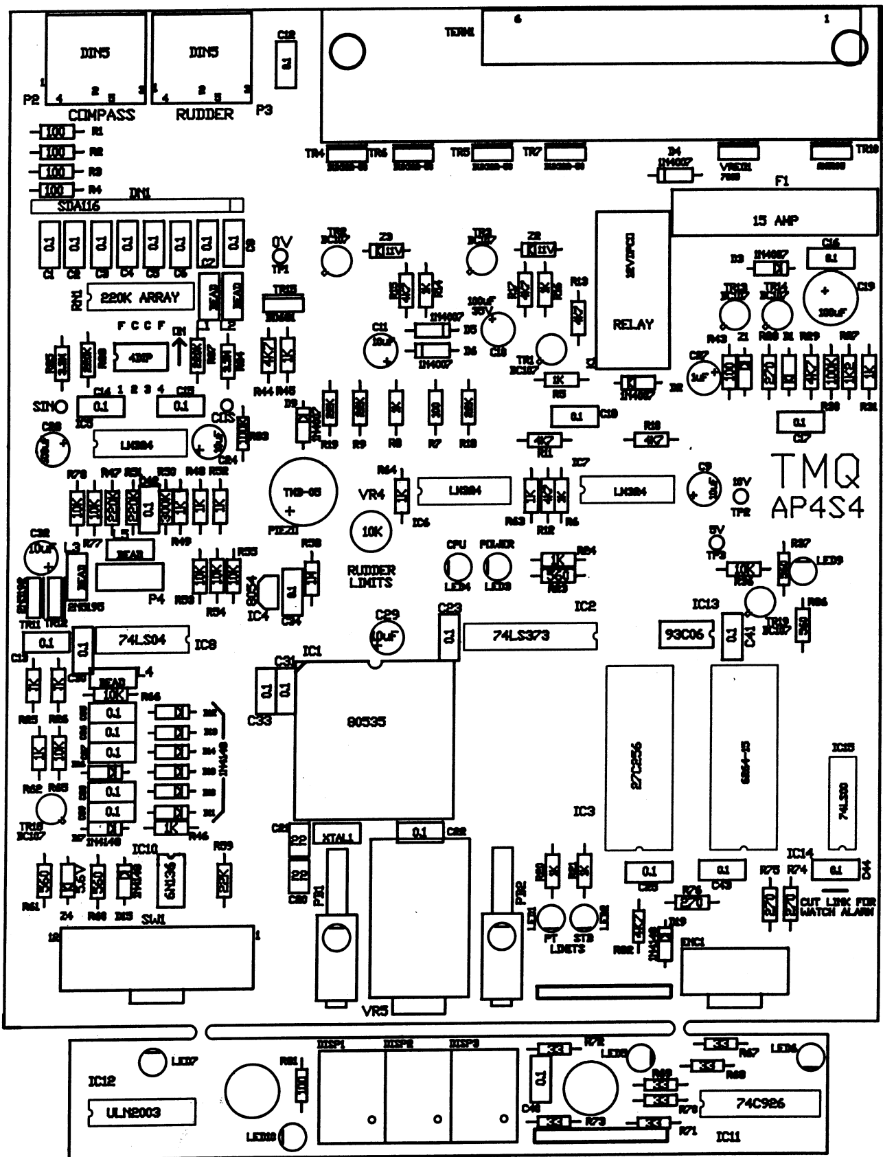
AP4S4 Top Overlay
