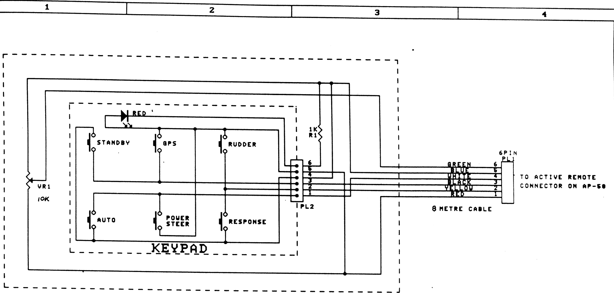
AP58 ACTIVE REMOTE UNIT, REAR VIEW
