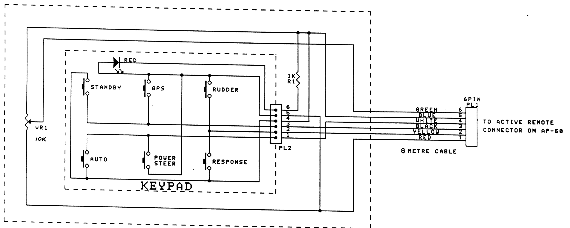
AP50 ACTIVE REMOTE UNIT, REAR VIEW
